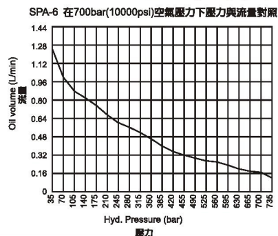
SPA-6 Pressure vs volume based on 700bar(10000psi) air pressure
